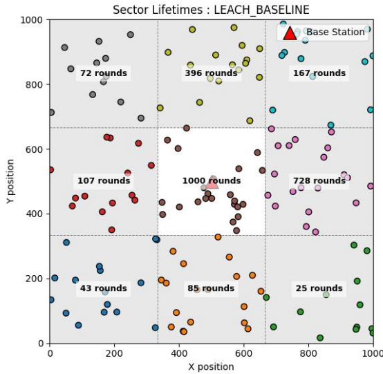
Fig 6.1 Sector-wise survival in LEACH
